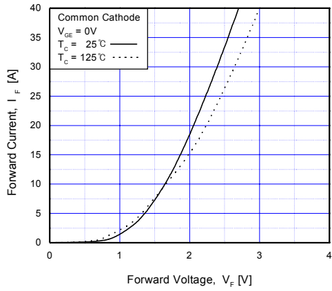
Fig 15. Forward Characteristics
